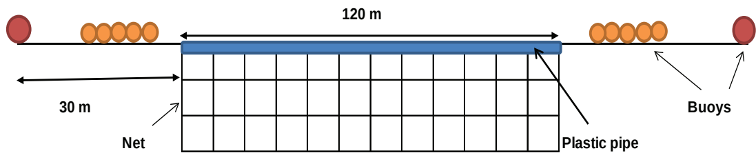
Figure 15 Long-line - nets. View from the side of mussel farm in Åland
