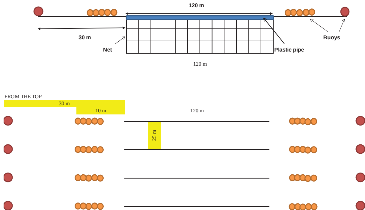
Figure 19; Visualisation of Åland farm
