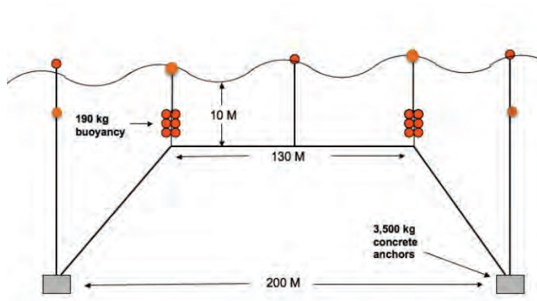
Figure 10 Open ocean mussel farm design.
