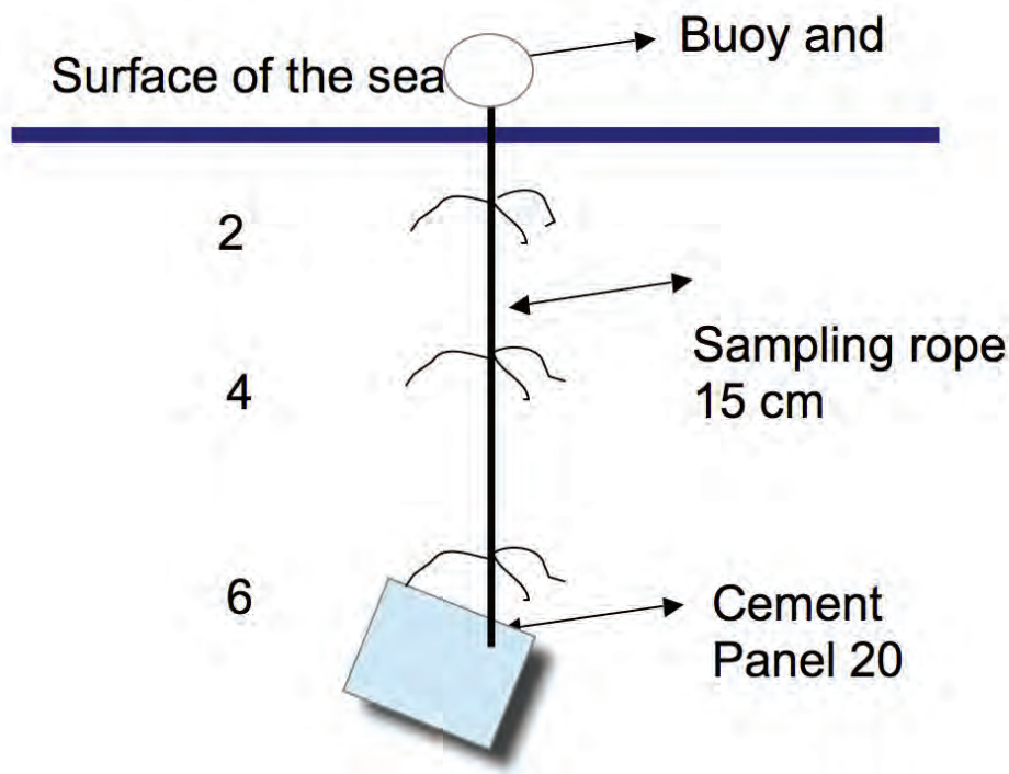
Figure 2. The scheme of one experimental unit used to assess the wave exposure and depths where mussels recruit better and grow faster. Three experimental units were set up in each of the 9 locations.
