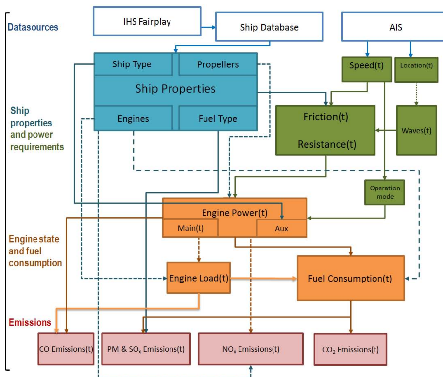
Fig. 1. A schematic diagram of the main components of the STEAM2 model and their inter-relations. The model input data sources are presented on the uppermost row of rectangles, and the model output data (i.e. emissions) are presented on the lowest row of rectangles. The arrows describe either the flow of information in the model, or a modelled dependency between various factors. The different colors denote the various categories of factors included in the model; dotted and solid arrows are used only for visual clarity.
